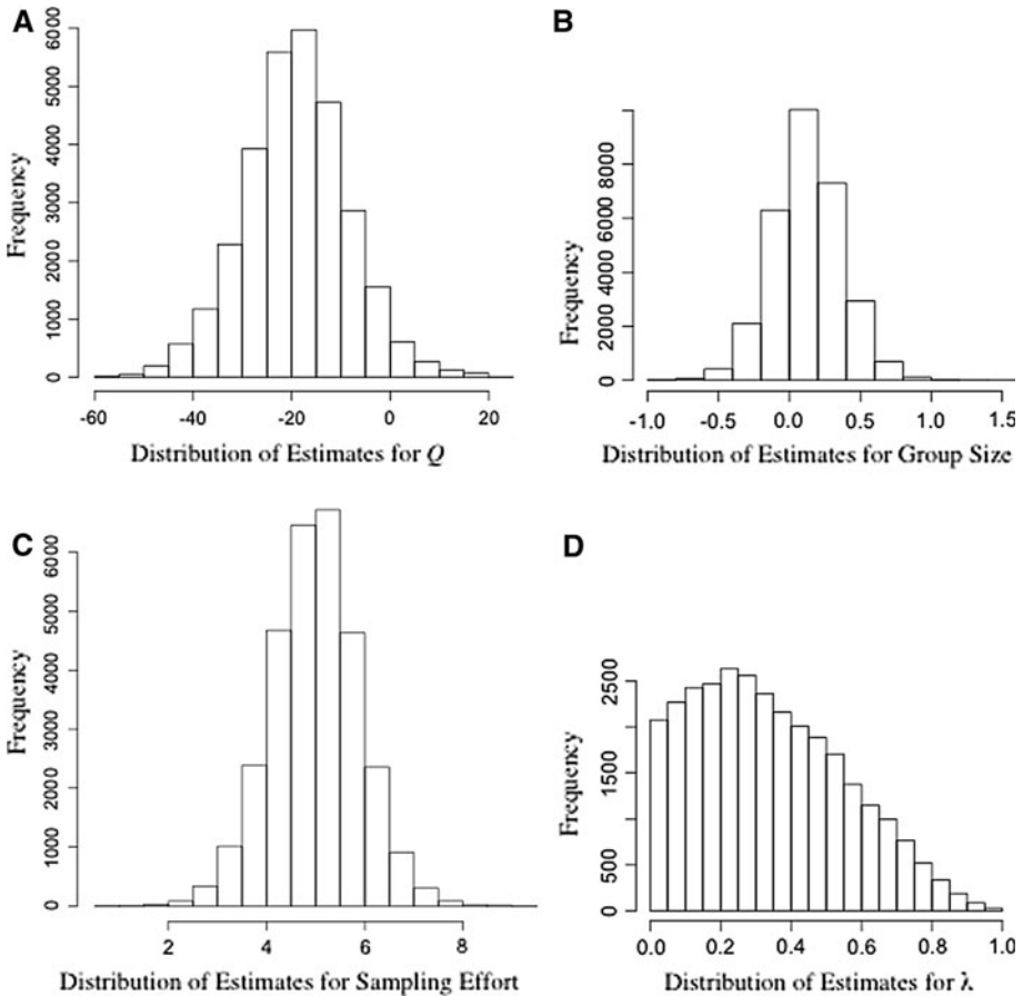
Fig. 3 Distributions of regression coefficients predicting the richness of closely-transmitted parasites of primates (panels A–C) and \lambda (panel D) (empirical results). Histograms represent the distribution of values sampled from the Bayesian (MCMC) analysis, controlling for phylogenetic uncertainty. For regression coefficients, an absence of an effect would be indicated by a histogram centered on zero, while increasingly strong effects are indicated by a departure from zero (e.g. for sampling effort)
