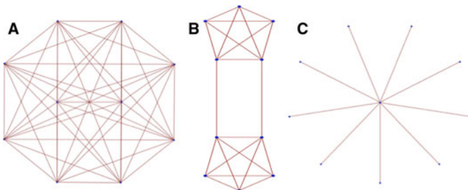
Fig. 1 Graphical representations of networks with extreme values of community modularity ( Q ) and the eigenvector centralization index ( C ). Network A is a complete network (i.e. an edge between every pair of nodes) with 10 nodes. Since there are no subgroups in Network A , Q = 0 , and since every node has the same number of edges, C = 0 . Network B also has 10 nodes, but is divided into two clear subgroups and thus has a high modularity, Q = 0.409 . Network C again has 10 nodes, but is a “star network,” which defines the maximum value of C = 1 ; one node, the most central node, has n-1 connections, while all other nodes have 1 connection
