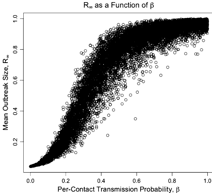
Fig. 2 Non-linear relationship between average outbreak size ( R_\infty ) in simulations and the per-contact transmission probability ( \beta ) across the full range of \beta
